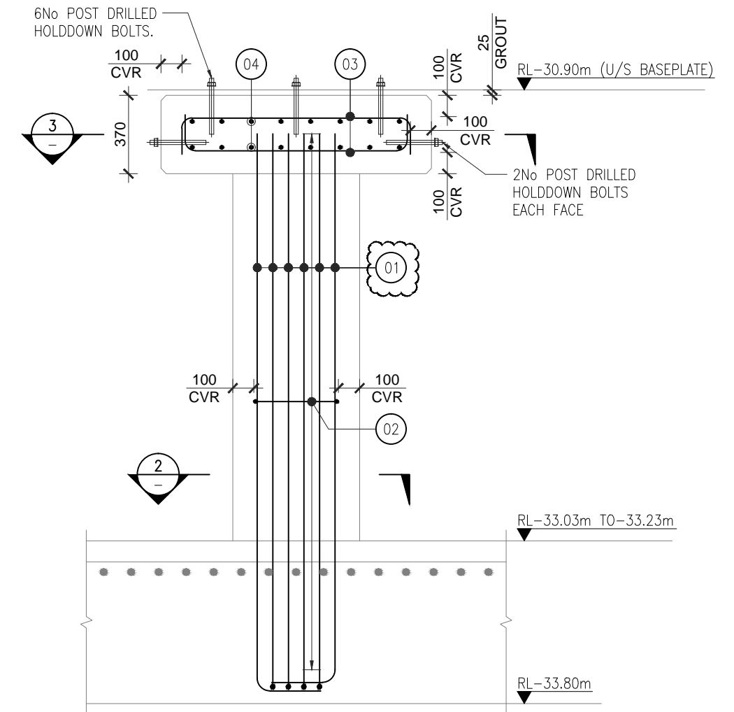
ELEVATION 2 PIPE SUPPORT CP2 (6No) SCALE: 1:25
