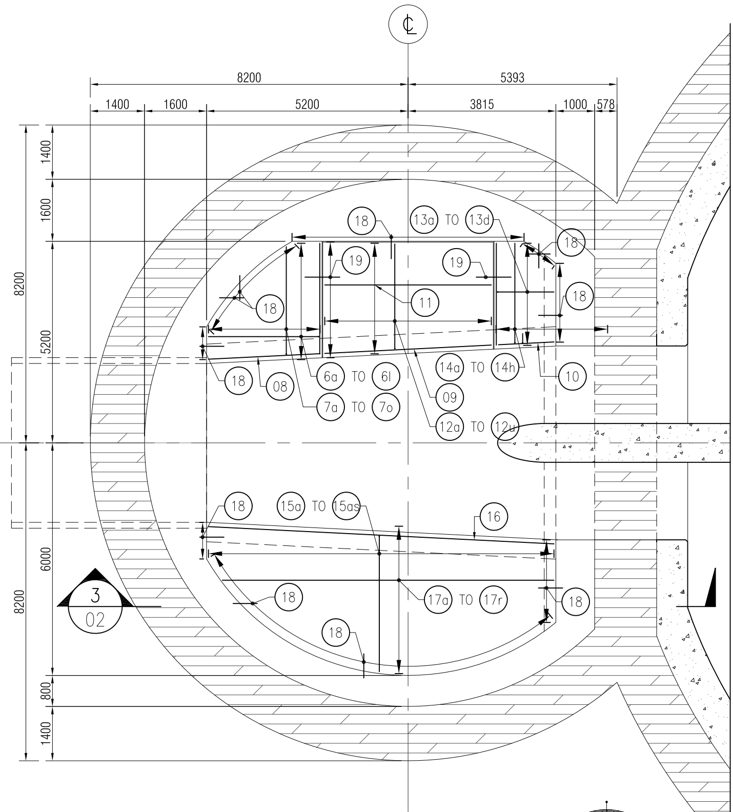
BASE SLAB BENCHING SLAB LAYOUT @ RL -25.05m SCALE: 1:100
