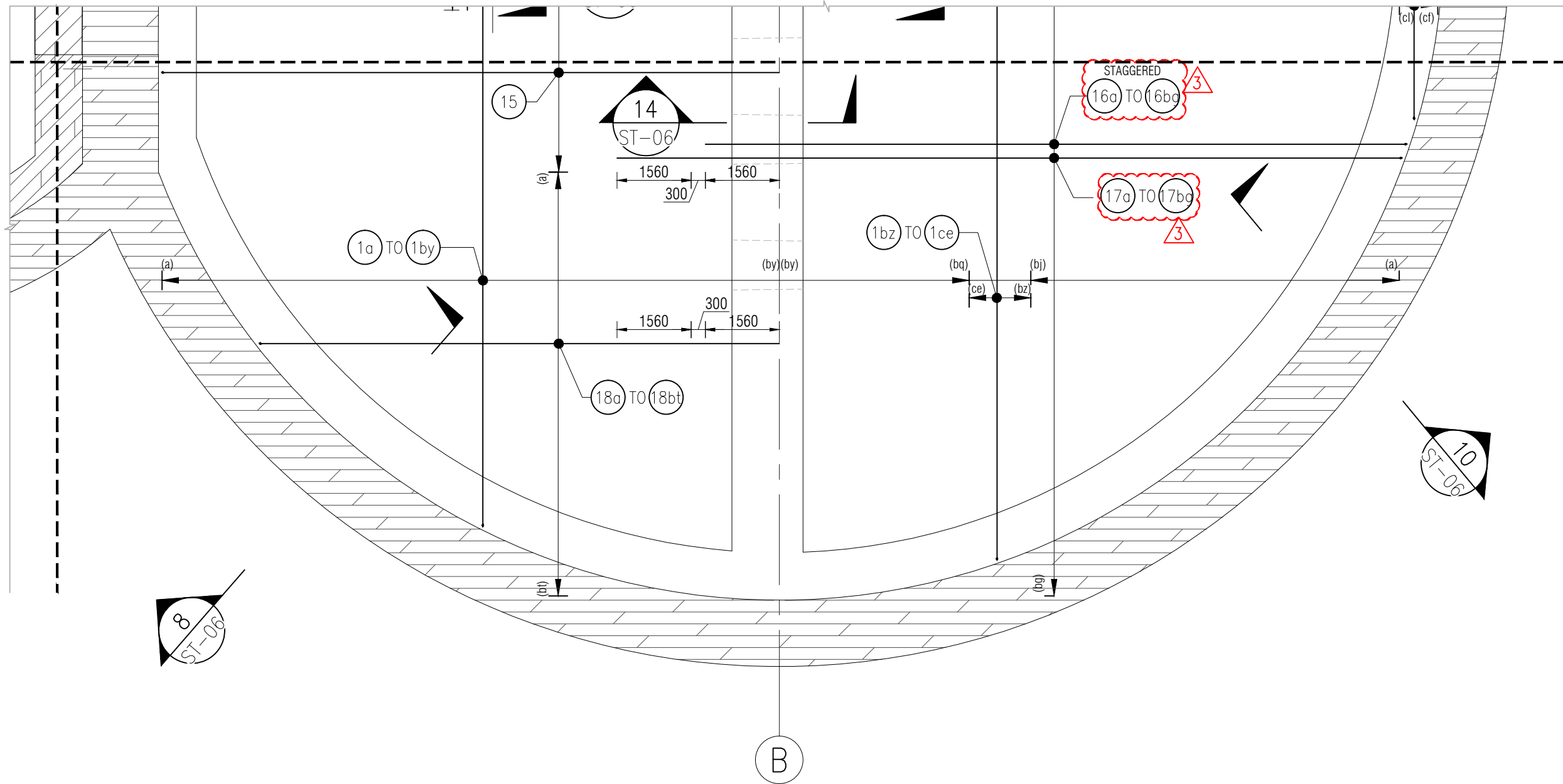
BASE SLAB TOP REINFORCEMENT DETAILS AT RL -33.80m SCALE 1:100
