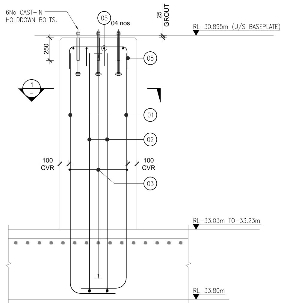
ELEVATION 1 PIPE SUPPORT CP1 (6No) SCALE: 1:25
