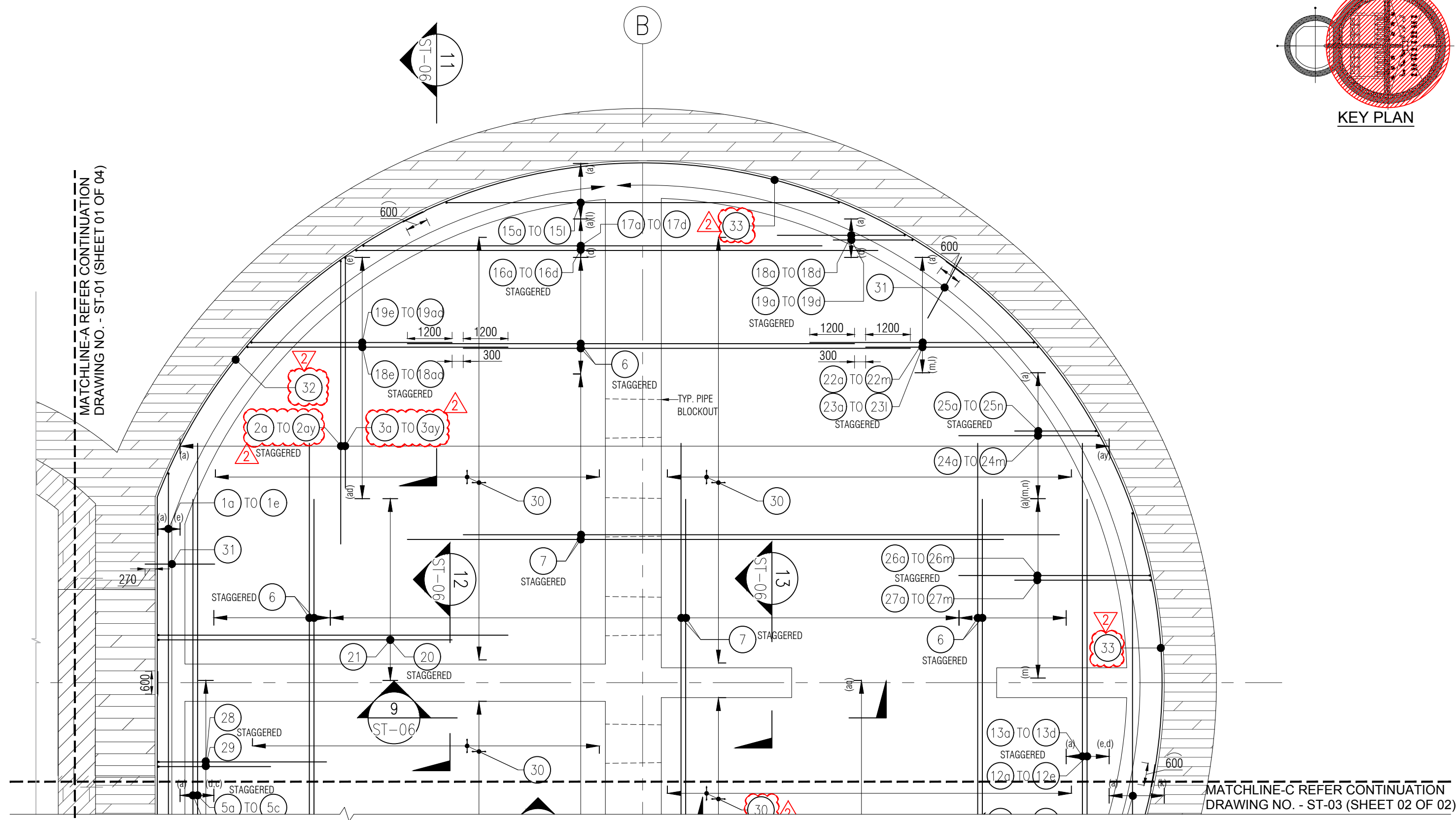
BASE SLAB BOTTOM REINFORCEMENT DETAILS AT RL -35.80m SCALE 1:100
