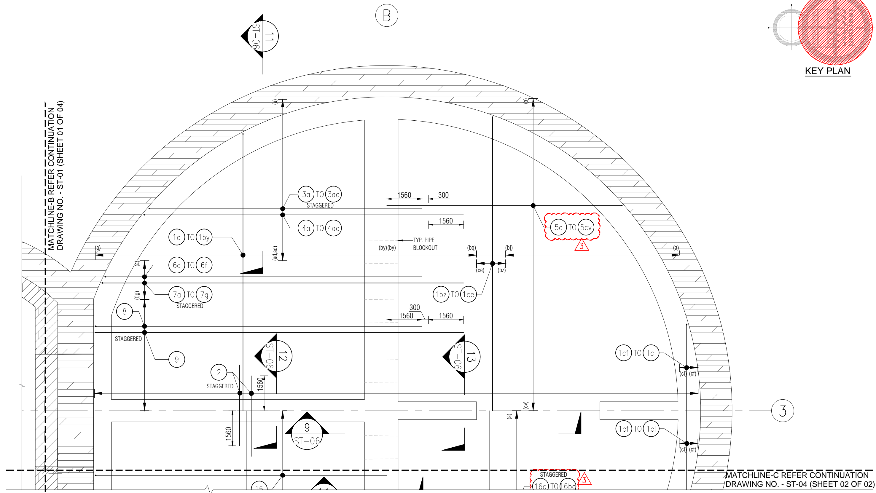
BASE SLAB TOP REINFORCEMENT DETAILS AT RL -33.80m SCALE 1:100
