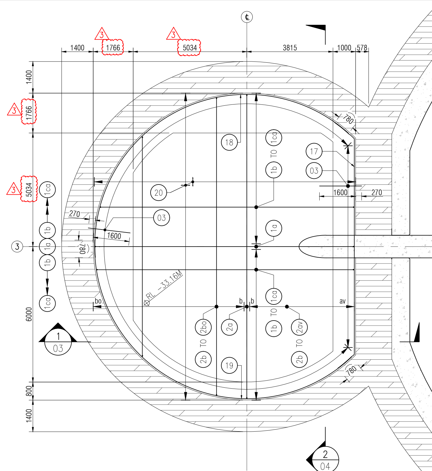
BASE SLAB BOTTOM LAYER (B1&B2) LAYOUT @ RL - 33.16M SCALE: 1:100
