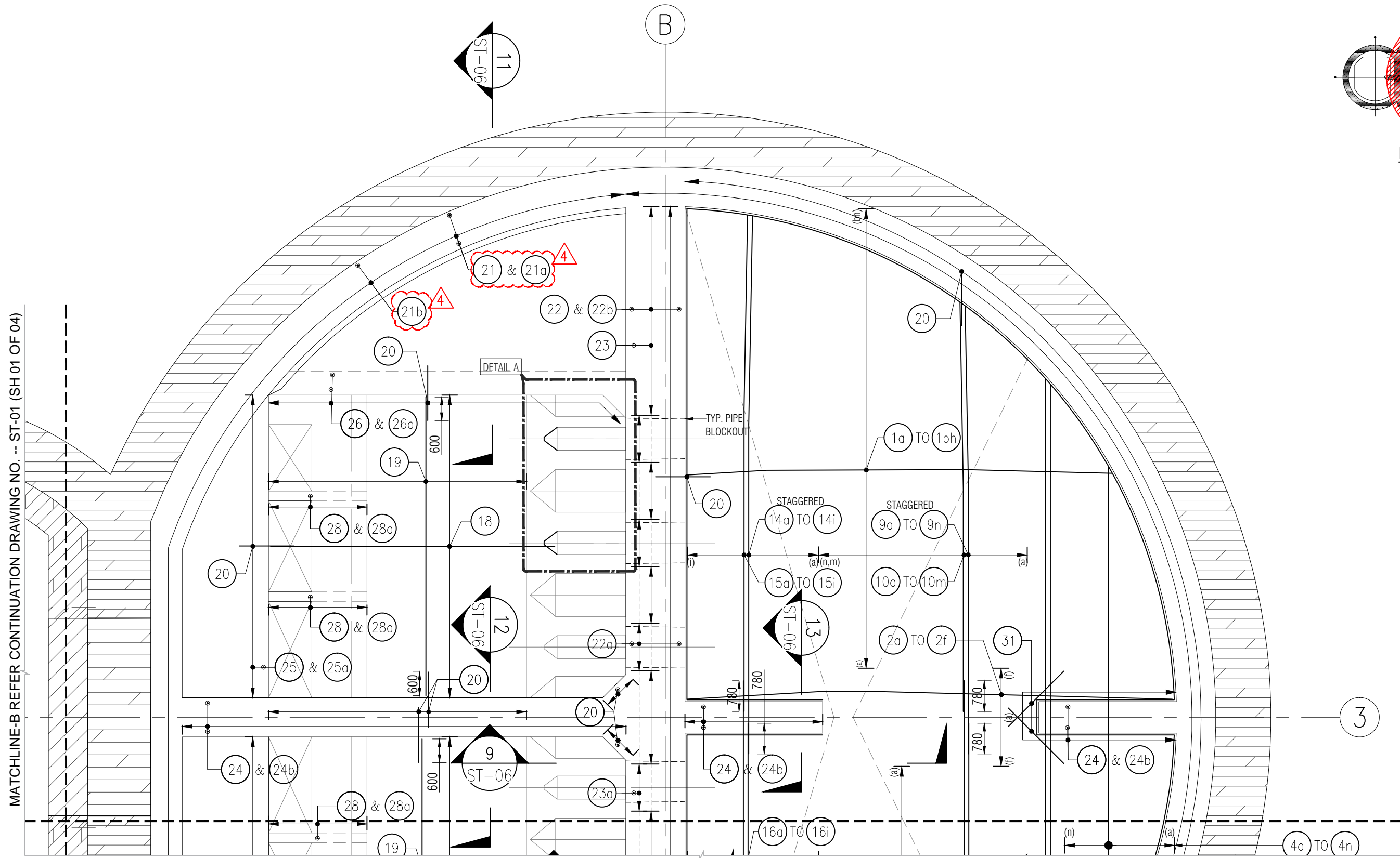
BASE SLAB TOP REINFORCEMENT DETAILS AT RL -33.03m SCALE 1:100
