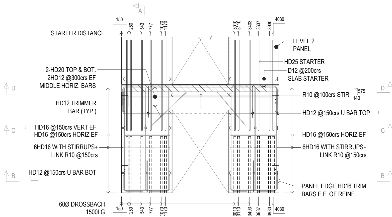
REO LAYOUT SCALE 1:50 VIEW FROM INSIDE
