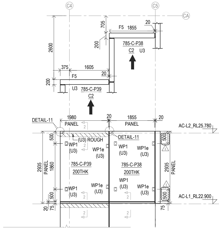
GRID CA+ PANEL ELEVATION (ELEVATION-C2)
