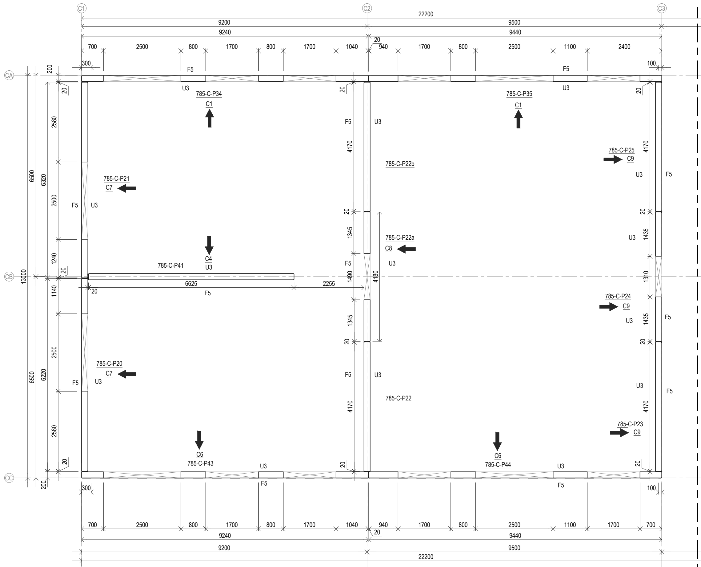
LEVEL 1 FLOOR PRECAST PANEL LAYOUT FOR BUILDING C
