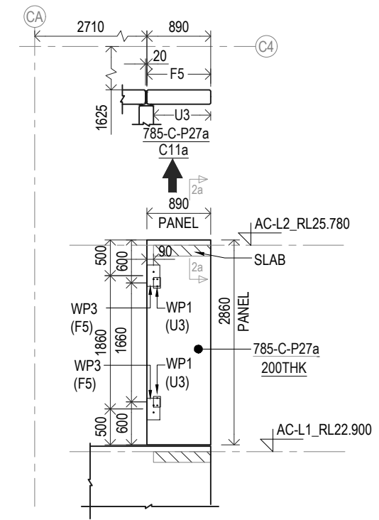
GRID C4+ PANEL ELEVATION (ELEVATION-C11a)
