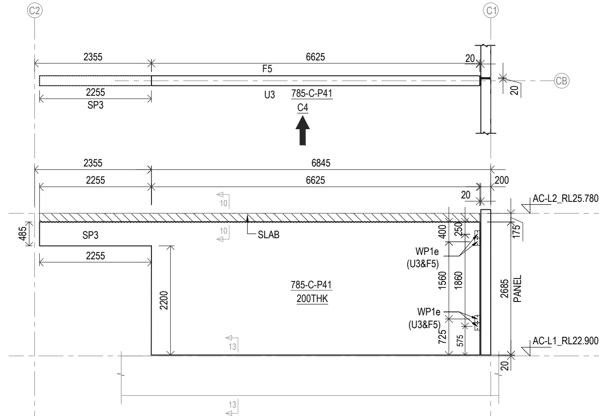
GRID CB/C1-C2 PANEL ELEVATION (ELEVATION-C4)
