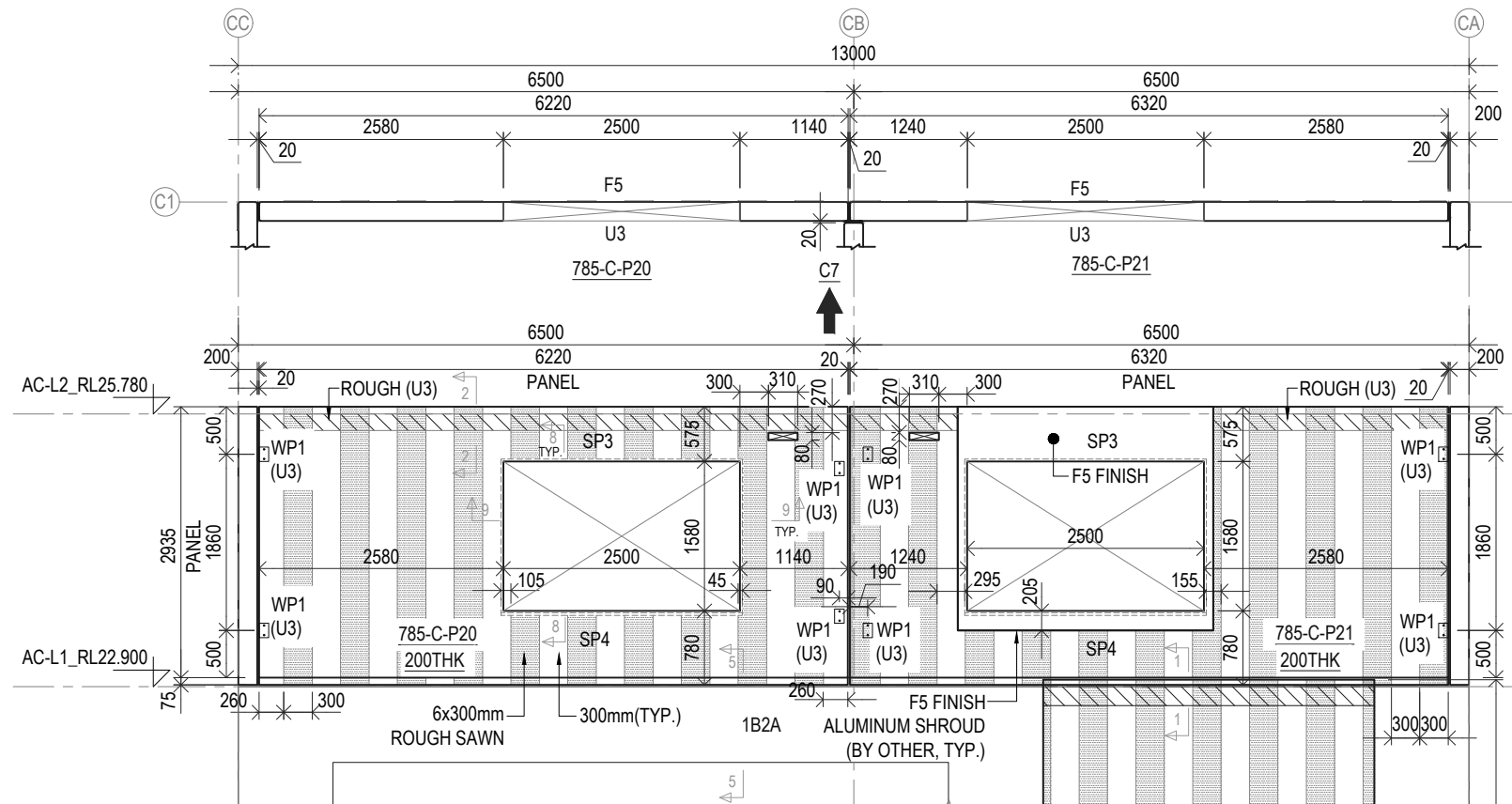
GRID C1 PANEL ELEVATION (ELEVATION-C7)
