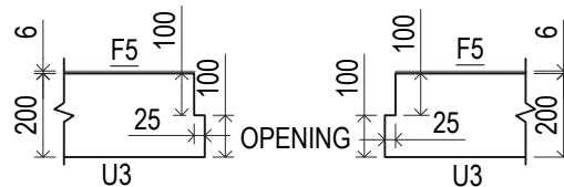
DETAIL - E
