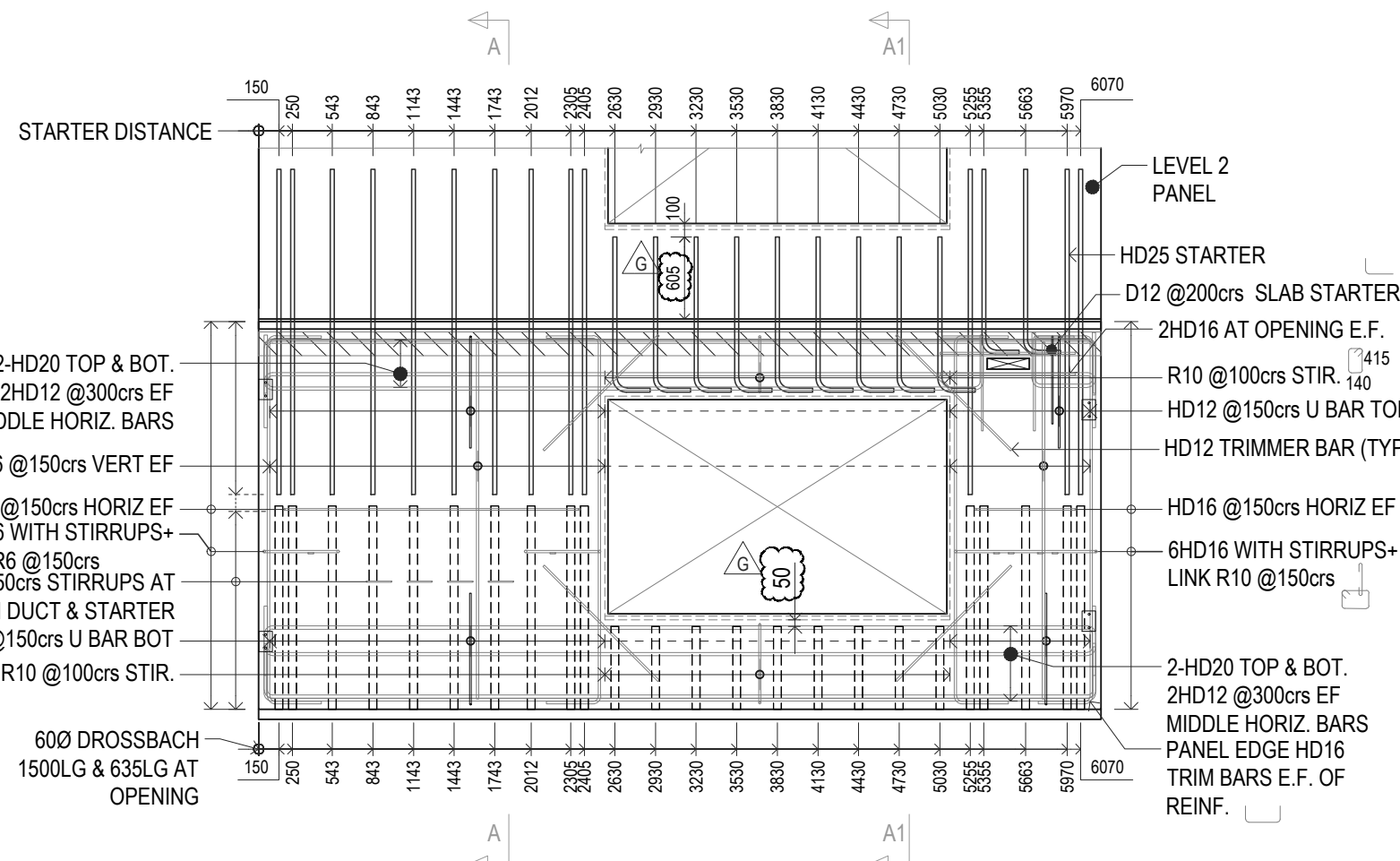
REO LAYOUT SCALE 1:50 VIEW FROM INSIDE
