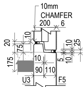
DETAIL - G
