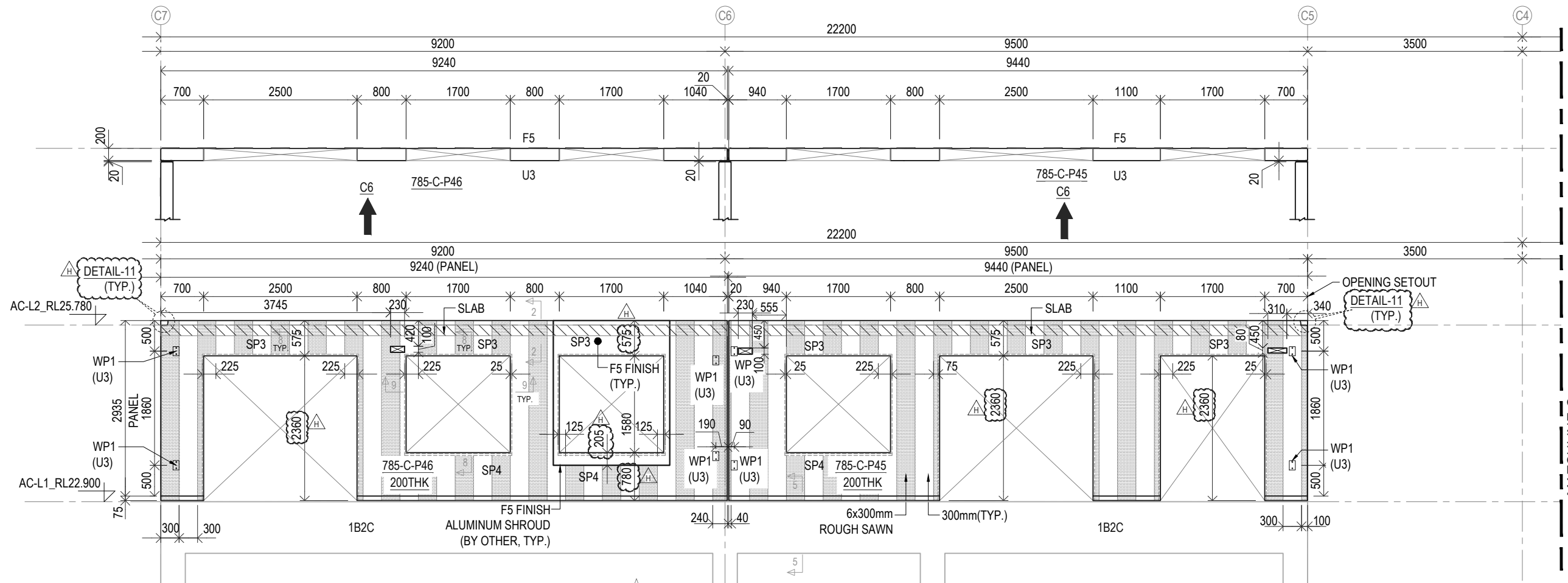
GRID CC PANEL ELEVATION (ELEVATION-C6)
