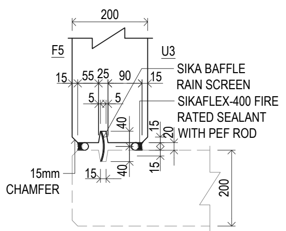
DETAIL - M (PRECAST PANEL JOINT PLAN DETAIL FOR GROOVE AT EDGE)
