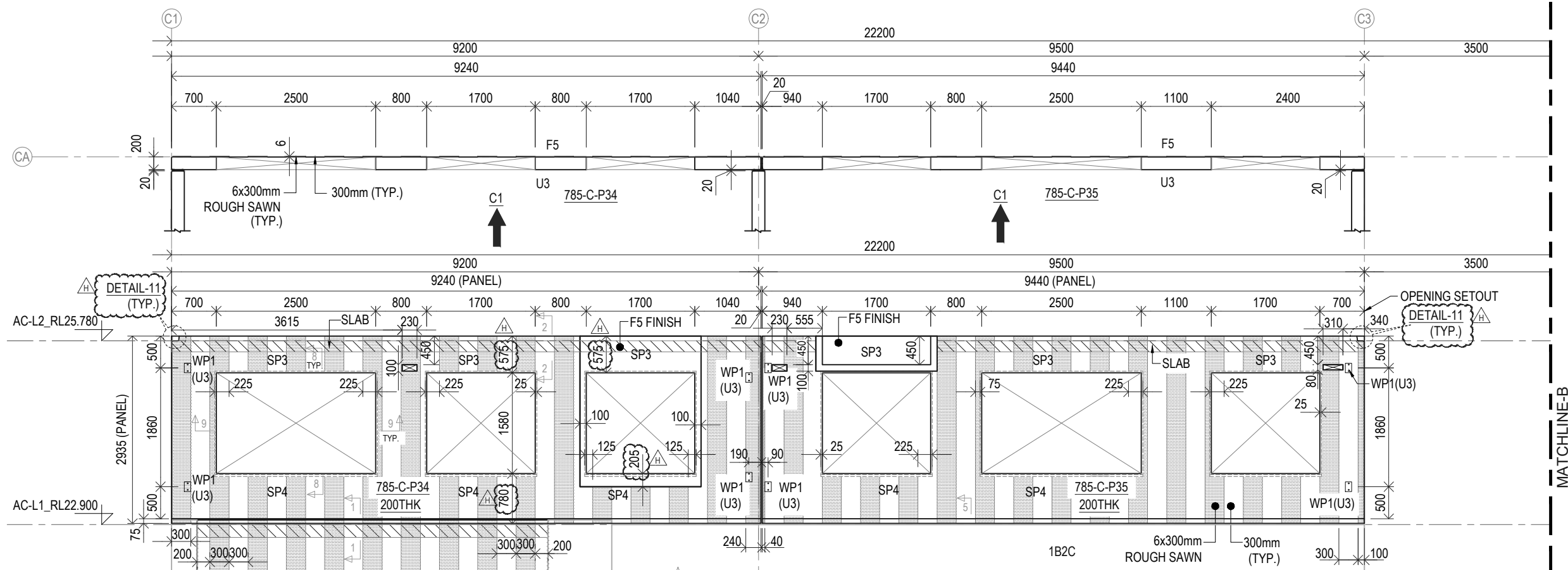
GRID CA PANEL ELEVATION (ELEVATION-C1)
