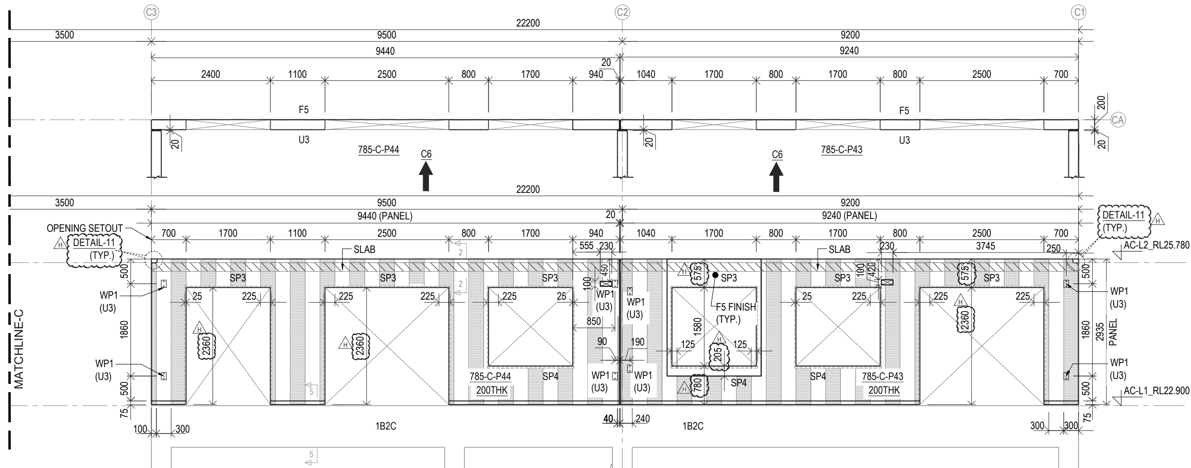
GRID CC PANEL ELEVATION (ELEVATION-C6)
