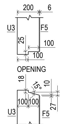
DETAIL - F
