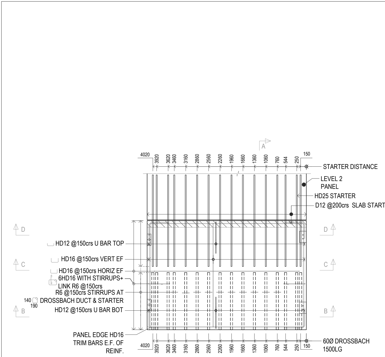
REO LAYOUT SCALE 1:50 VIEW FROM INSIDE
