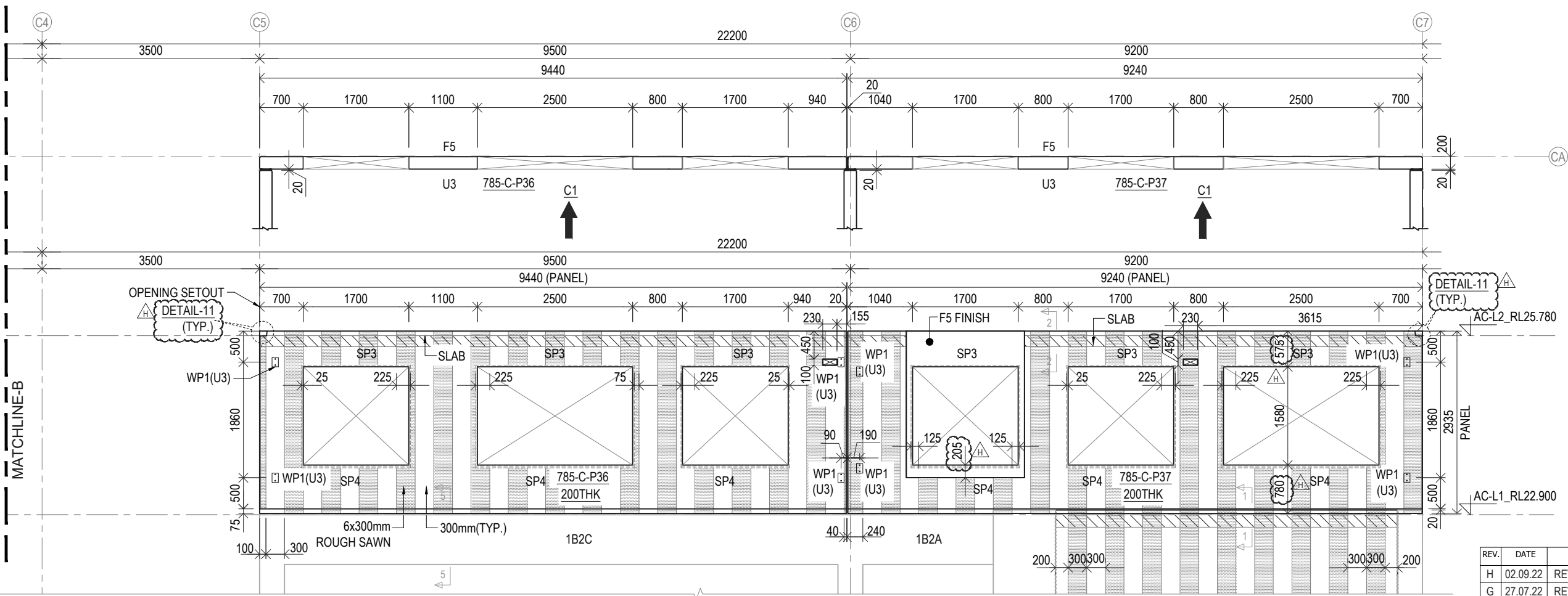
GRID CA PANEL ELEVATION (ELEVATION-C1)
