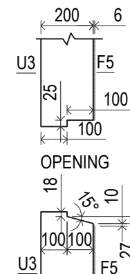
DETAIL - F
