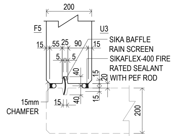
DETAIL - M (PRECAST PANEL JOINT PLAN DETAIL FOR GROOVE AT EDGE)
