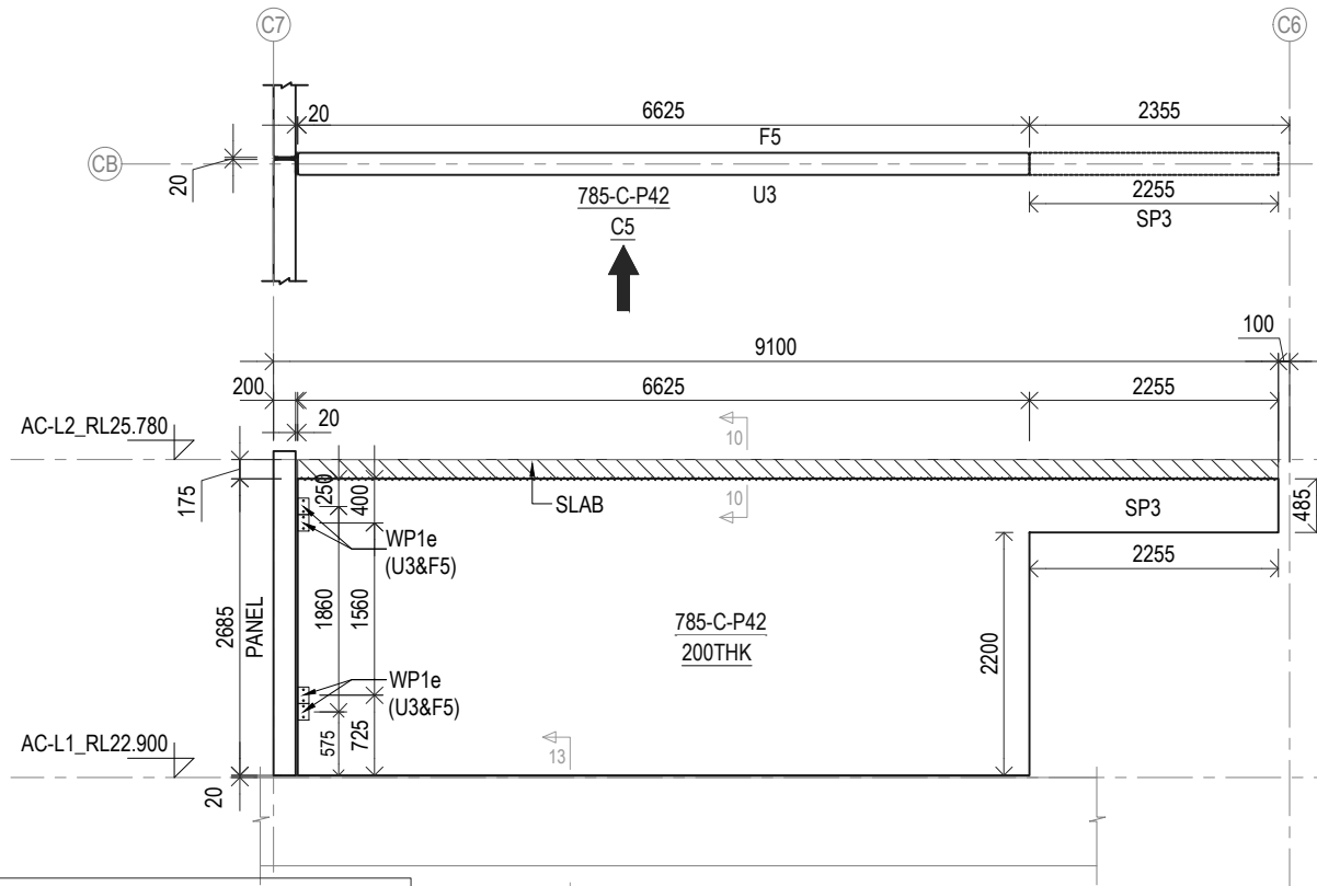
GRID CB/C6-C7 PANEL ELEVATION (ELEVATION-C5)
